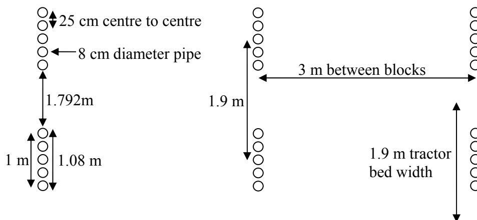
Figure 4.3. Trial layout diagram: small circles represent the pipes sunk into the ground, only three out of five blocks are shown.
